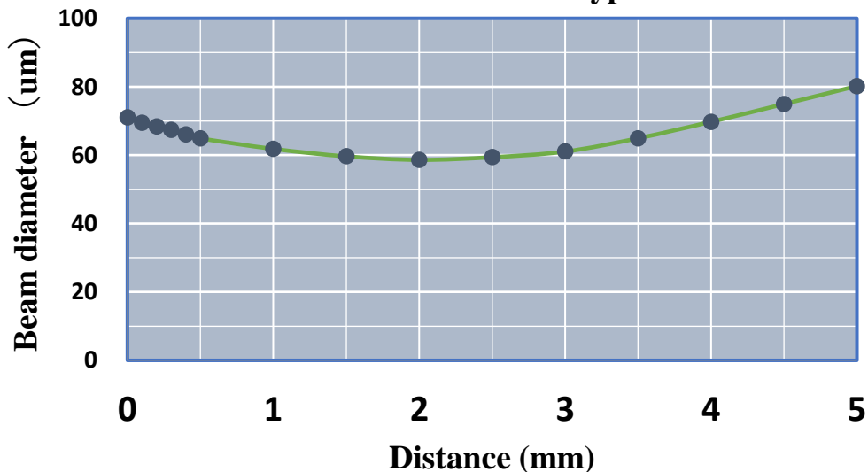
Beam waist @633 nm of LC type collimator
