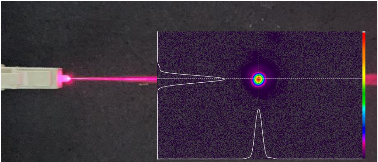
Beam waist @633 nm of LC type collimator
