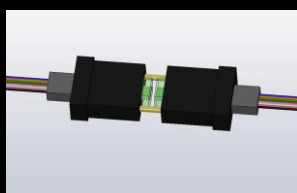
EB-MT connector for immersive cooling
